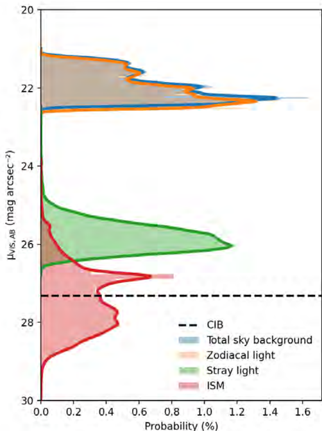
Fig. 7. Distribution of sky background surface brightness in the Euclid /VIS exposures as predicted by the IRSA model for the zodiacal light (orange), interstellar medium (ISM, red), and the cosmic infrared background (CIB, black dashed line), the simulations for the average stray-light contamination (green), and the combination of all components (blue histogram).
