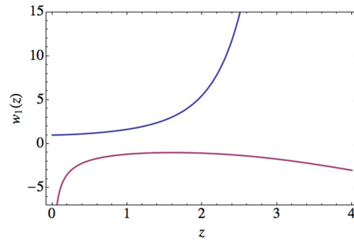
Figure 18. The two PV transcendents w_1(z) given by equations (11.11) belonging to the exponential hierarchy.
